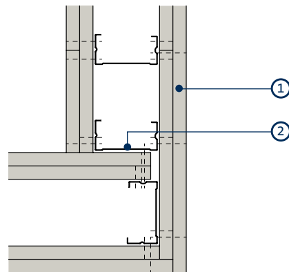
Corner detail - double layer
